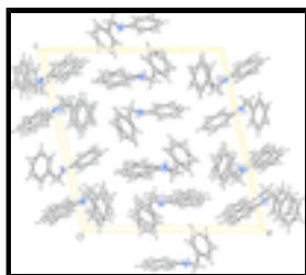
Fig. 3. Molecular packing of the title compound, viewed along [010] (anisotropic displacement ellipsoids drawn at 50% probability level).
